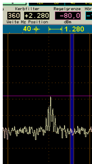
Settings and display of the notch filter.
