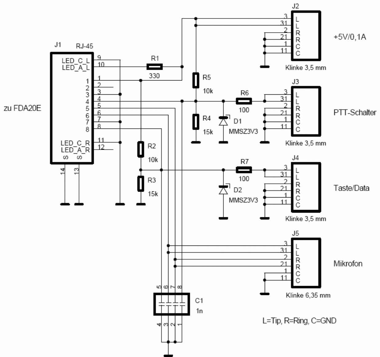
Internal circuitry of the adapter MAB5A
